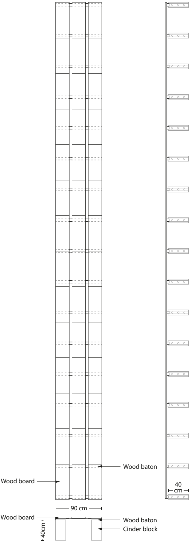
Technical drawing
